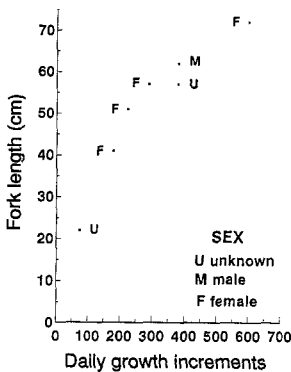
Fig. 7. Daily growth increments for S. commerson .
