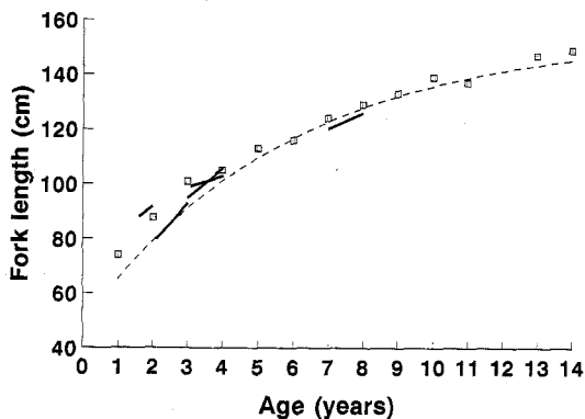
Fig. 10. Growth increments from tagging (solid lines) for known-age females of S. commerson , compared with the von Bertalanffy growth curve (dashed line) and mean observed length-at-age data (squares).
