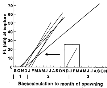
Fig. 8. Back-calculation of daily growth increments and fork length to month of spawning for S. commerson . In the box, a single short-term growth increment is offset by 12 months.
